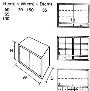
④ Double wall-mounted unit
